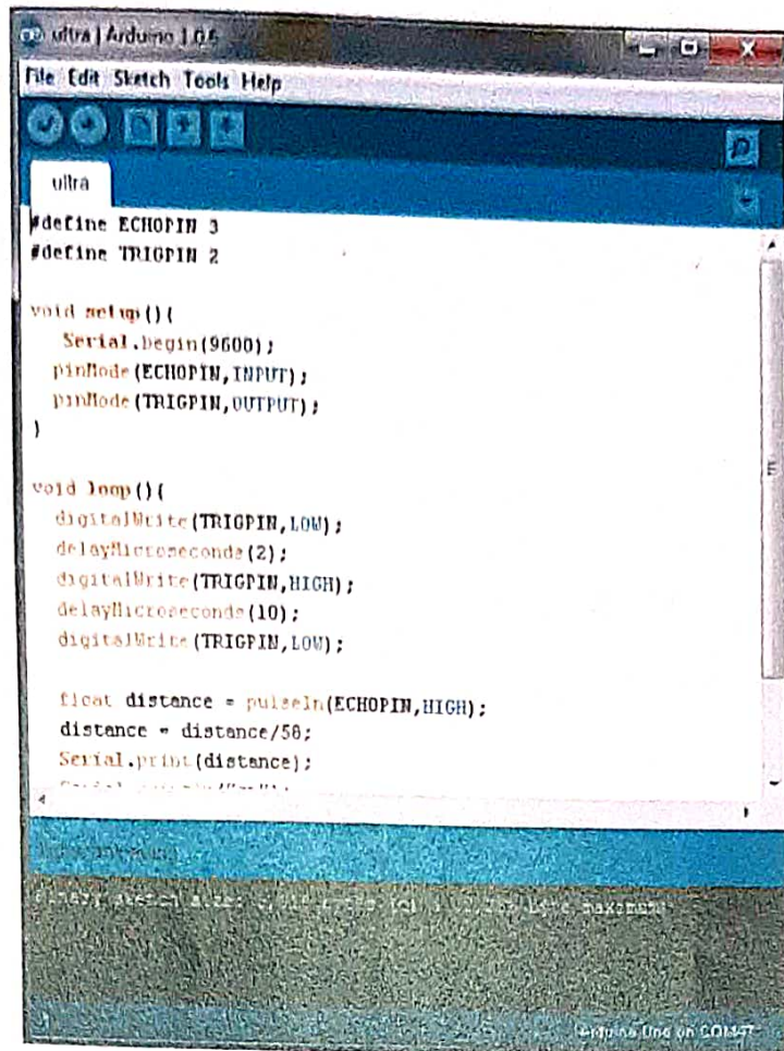
Figure No. 4.1.2b Arm Unit code
