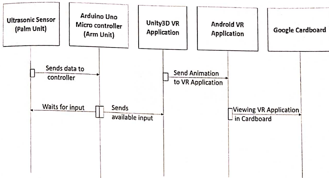
Figure No. 3.2.2 Sequence Diagram
